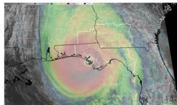
Hurricane Michael Source: NOAA/NWS https://www.weather.gov/tae/20181010_Michael
